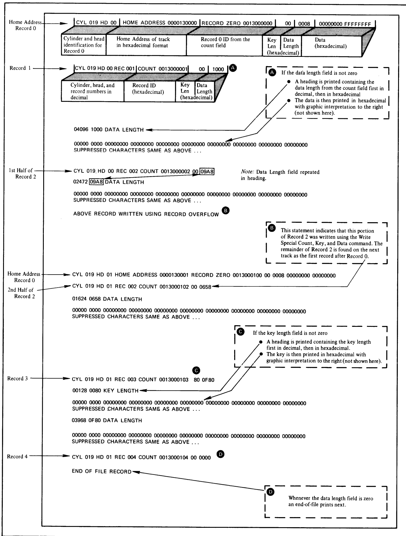
Figure 8. Annotated Sample of Output from the TYPE and PRINT Functions of the DDR Program
