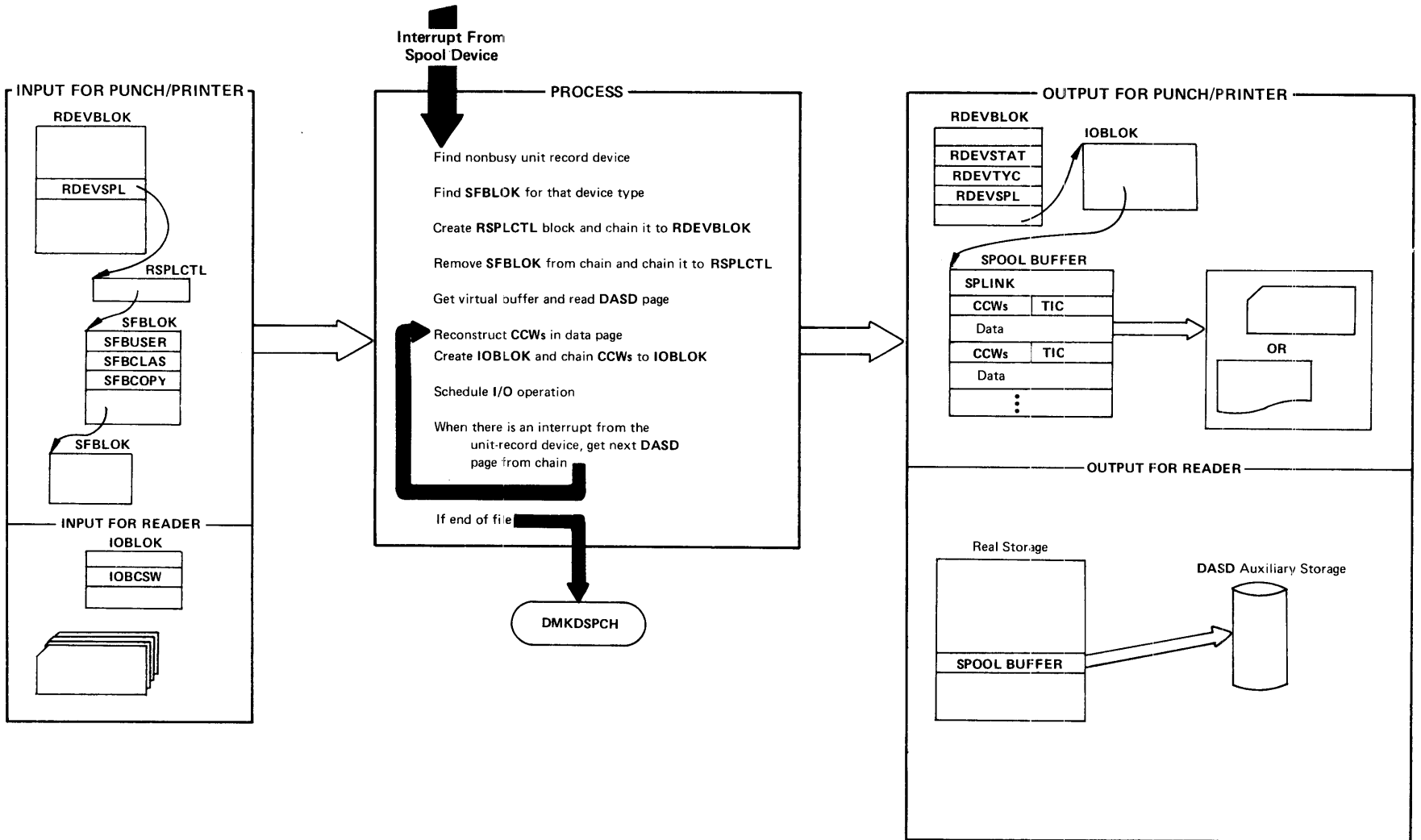
Figure 25. Real Spooling
