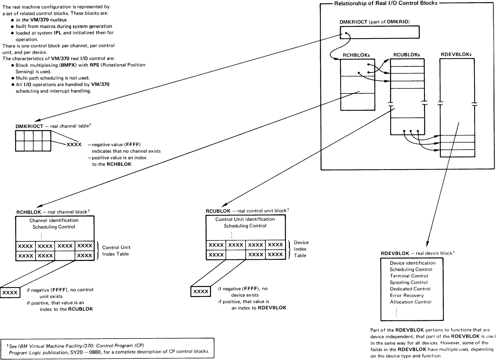
Figure 18. Real I/O Control Blocks
