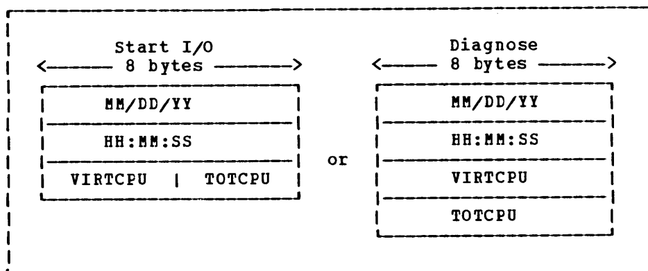
Figure 29. Formats of Pseudo Timer Information
