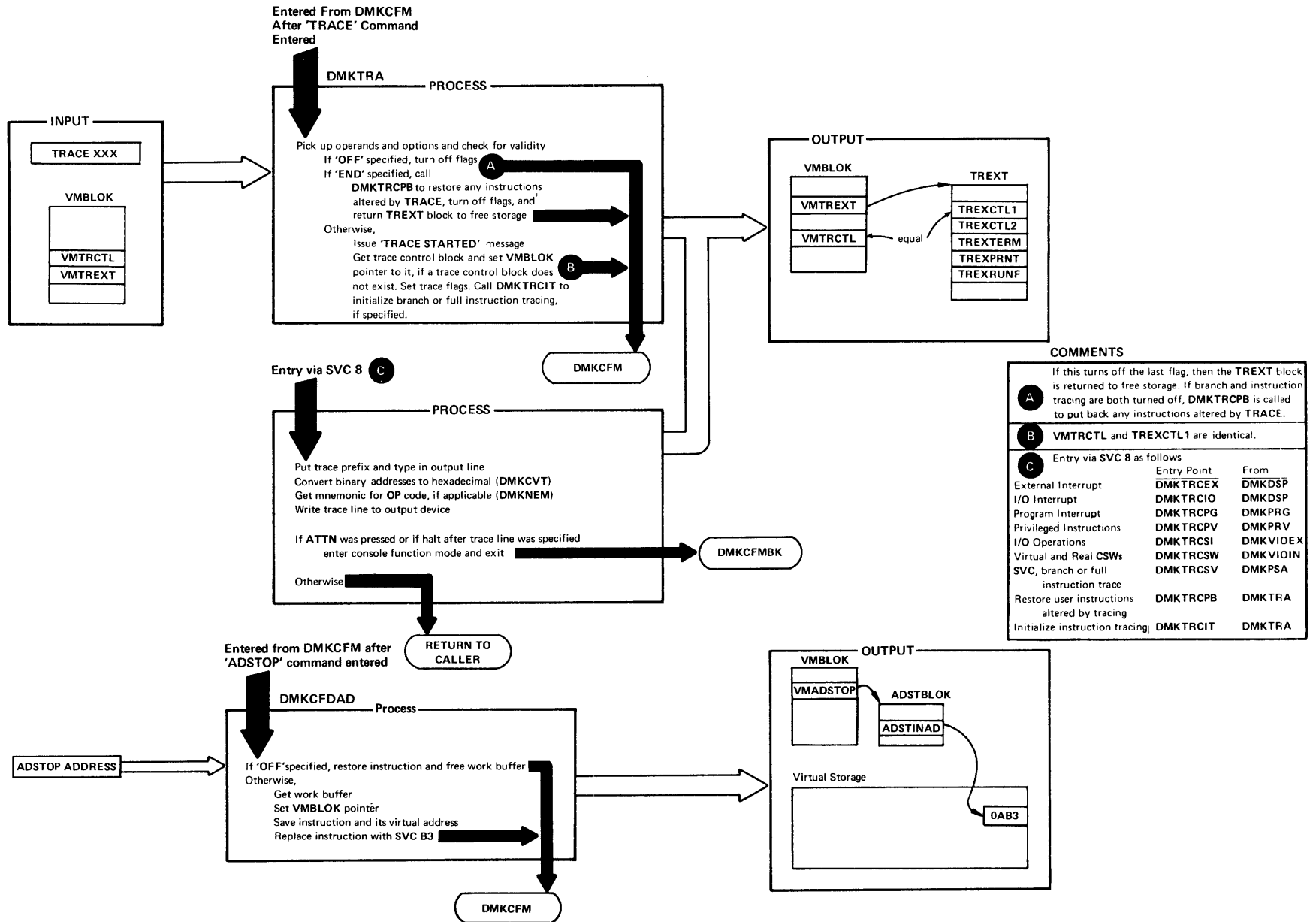
Figure 26. Virtual Tracing
