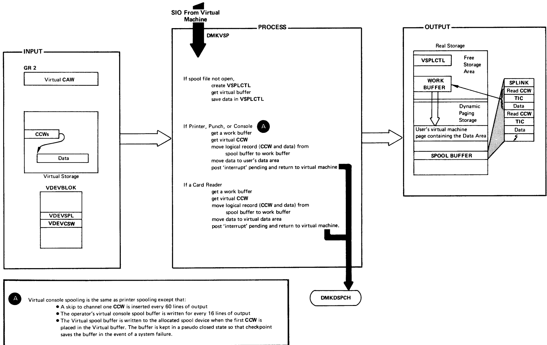
Figure 24. Virtual Spooling
