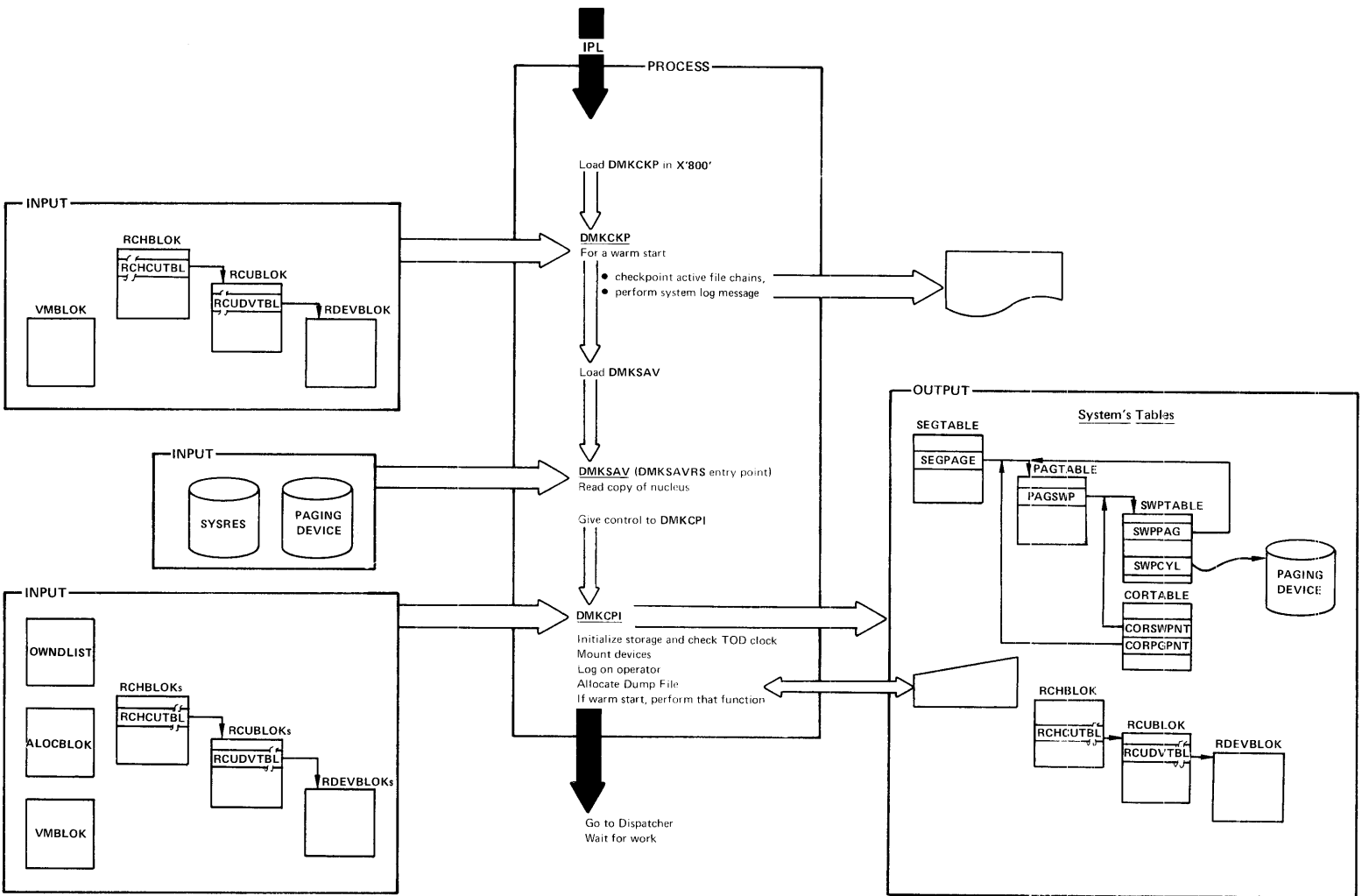
Figure 17. CP Initialization
